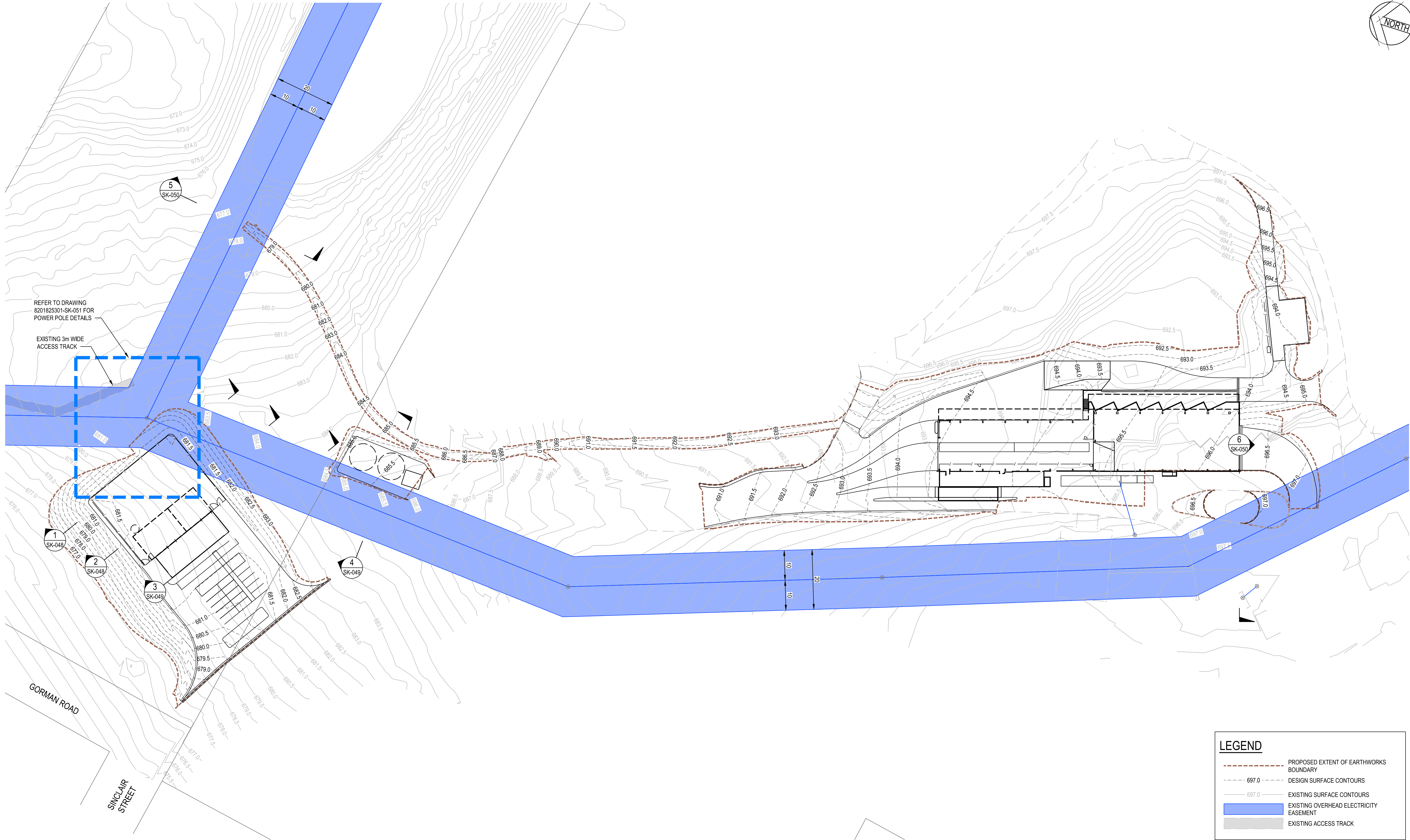
EXISTING ELECTRICAL EASEMENT LAYOUT SCALE 1:600
