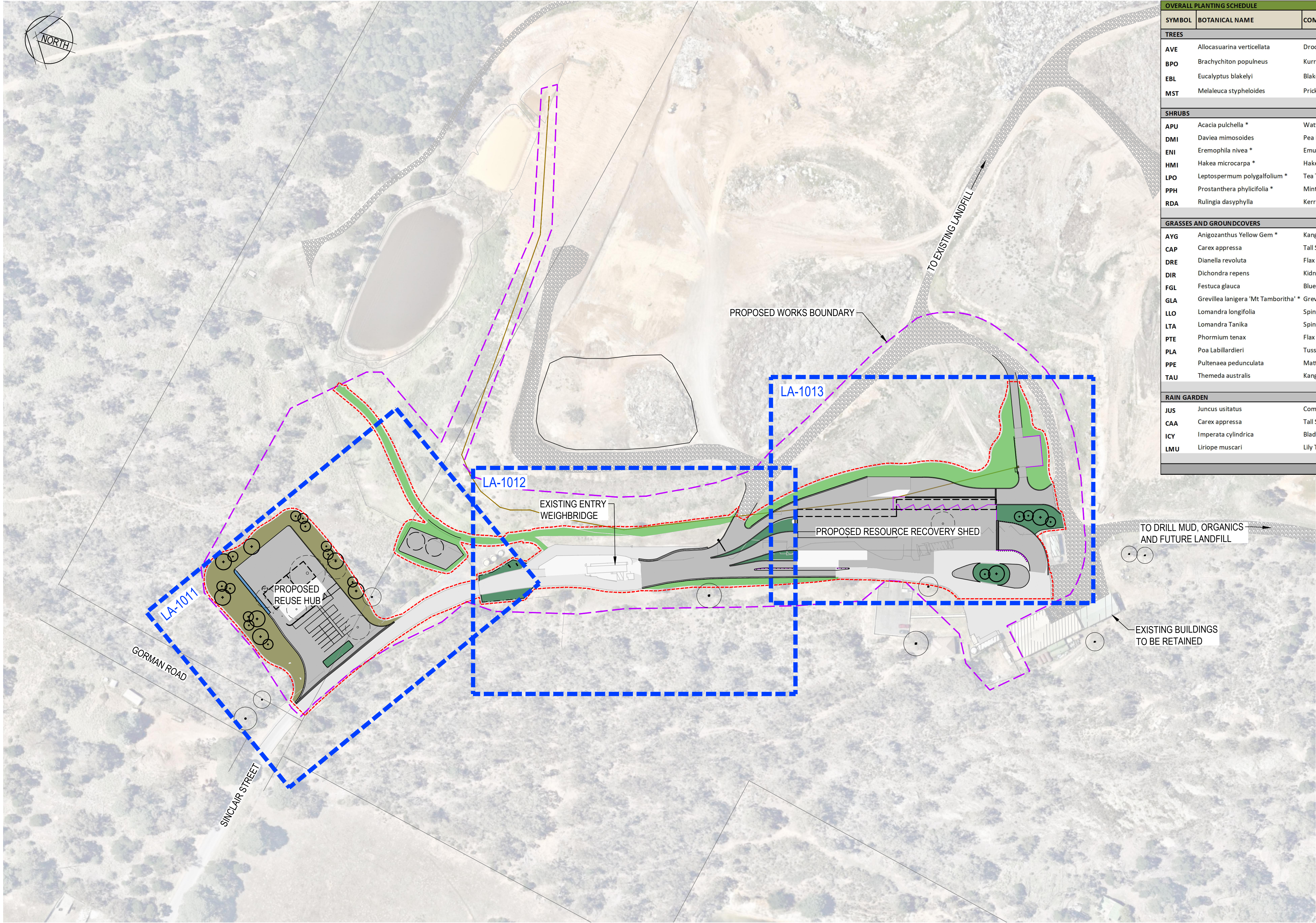
KEY PLAN SCALE 1:1000
