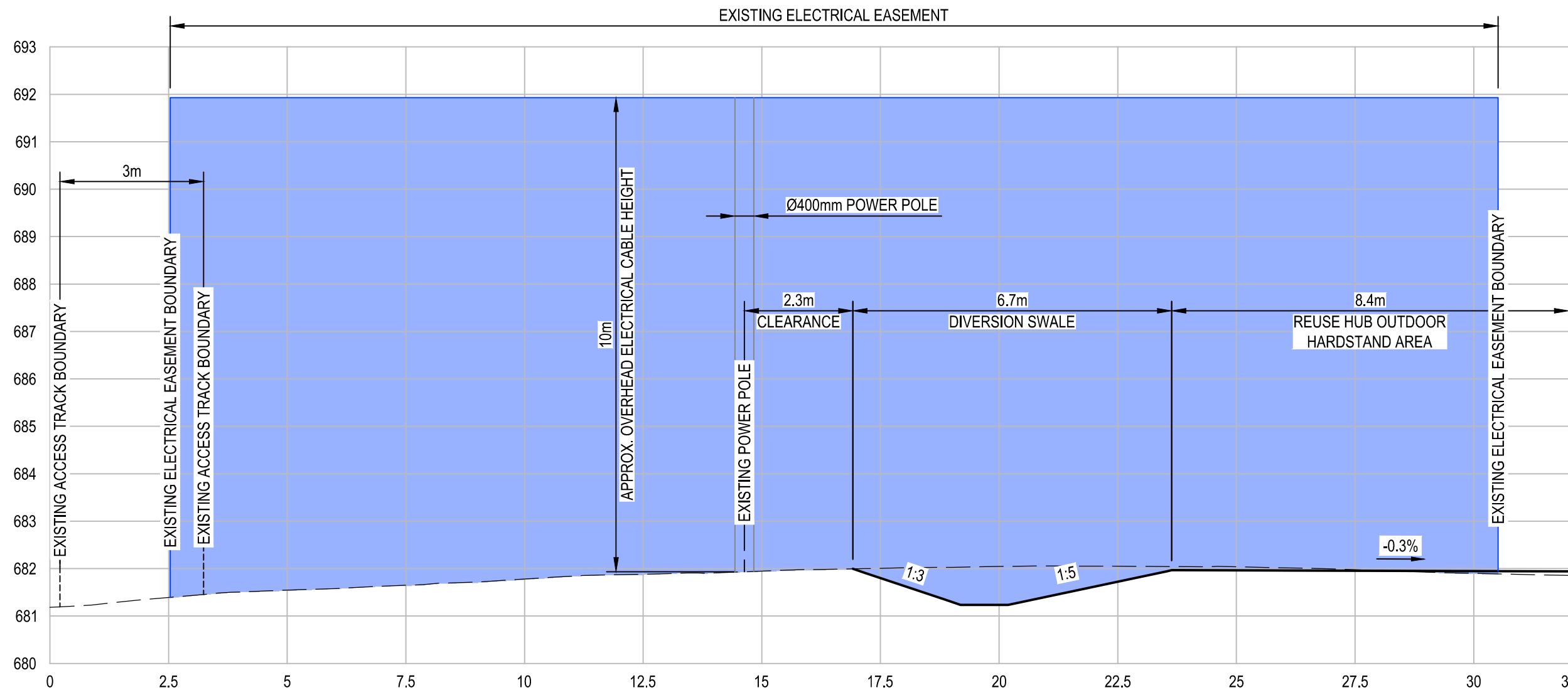
SECTION 7 SCALE 1:100
