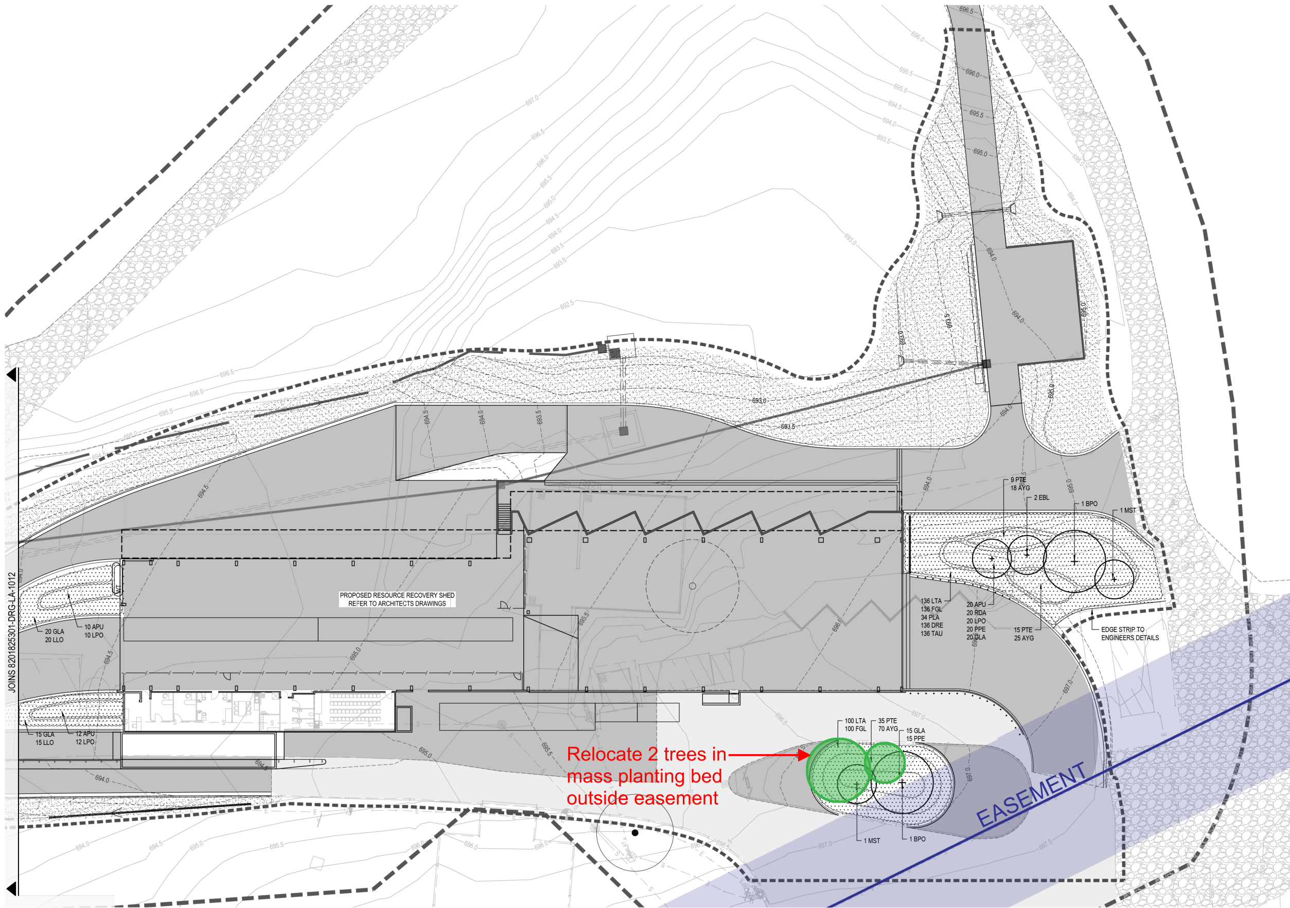
FINISHES, GRADING AND PLANTING PLAN SCALE 1:250
