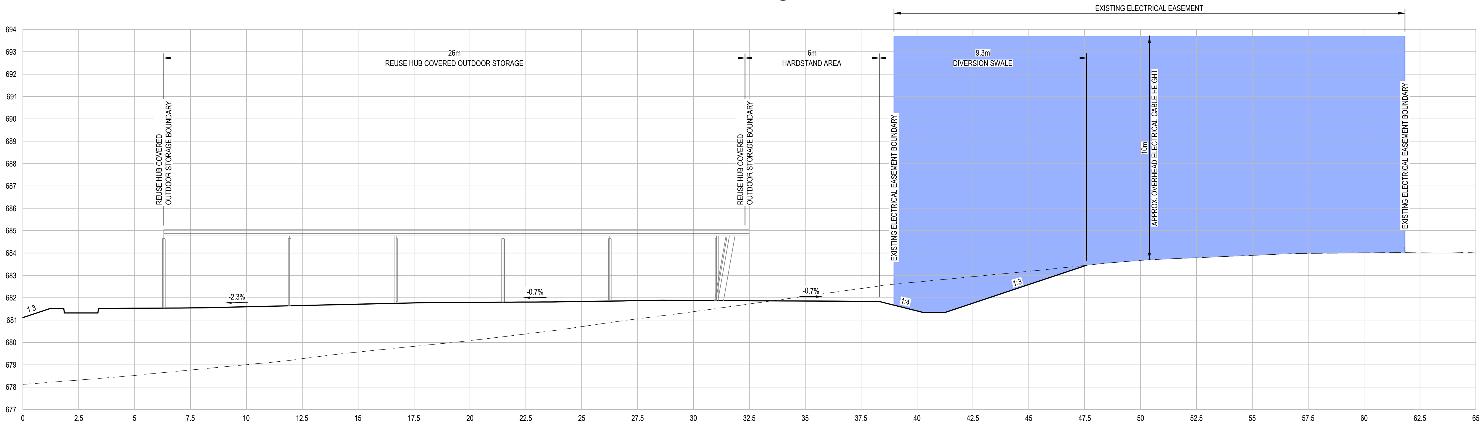
SECTION 2 SCALE 1:100
